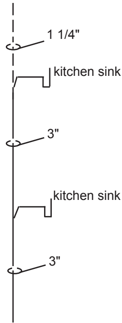
Figure 72. KS/KS stack
