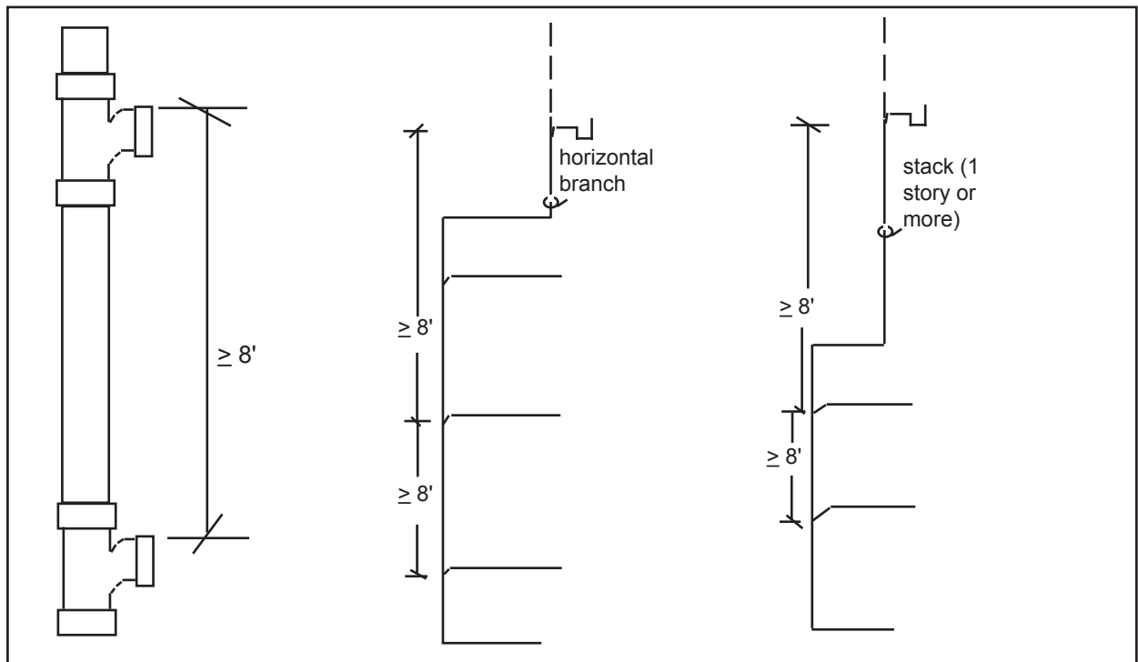
Figure 6. Branch Interval
