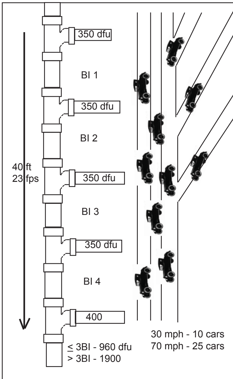
Figure 10 Capacity of stacks
