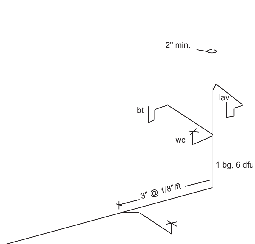
Figure 73. Combination drain and vent system
