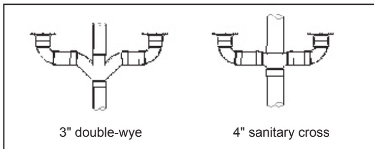
Figure 26. Back-to-back fixture drain connections.
