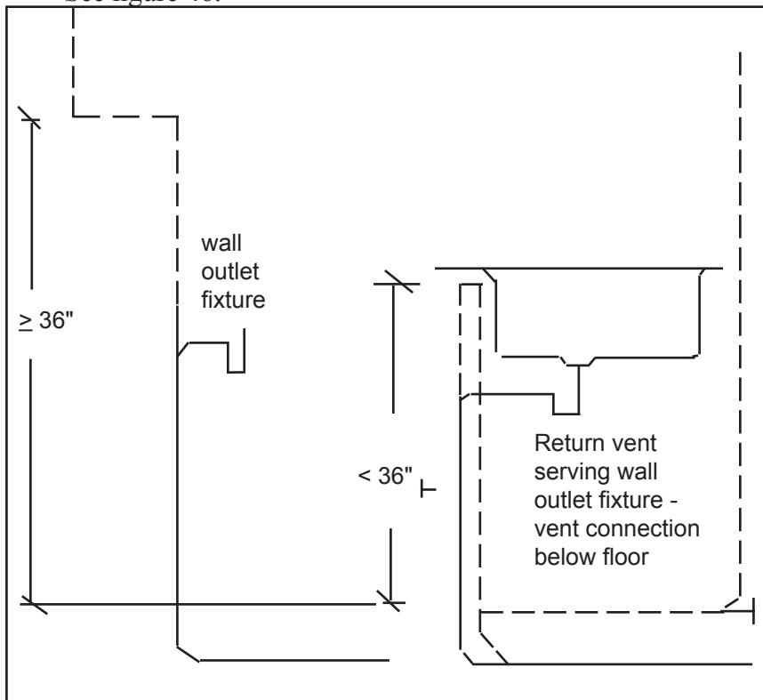
Figure 46. Vent offset height requirement.
