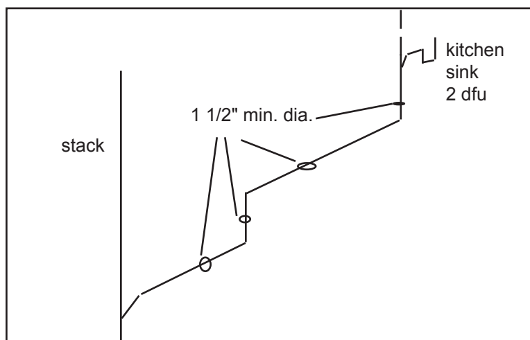
Figure 4. Sizing drains other than stacks.-Column 2 Table 82.30-2
