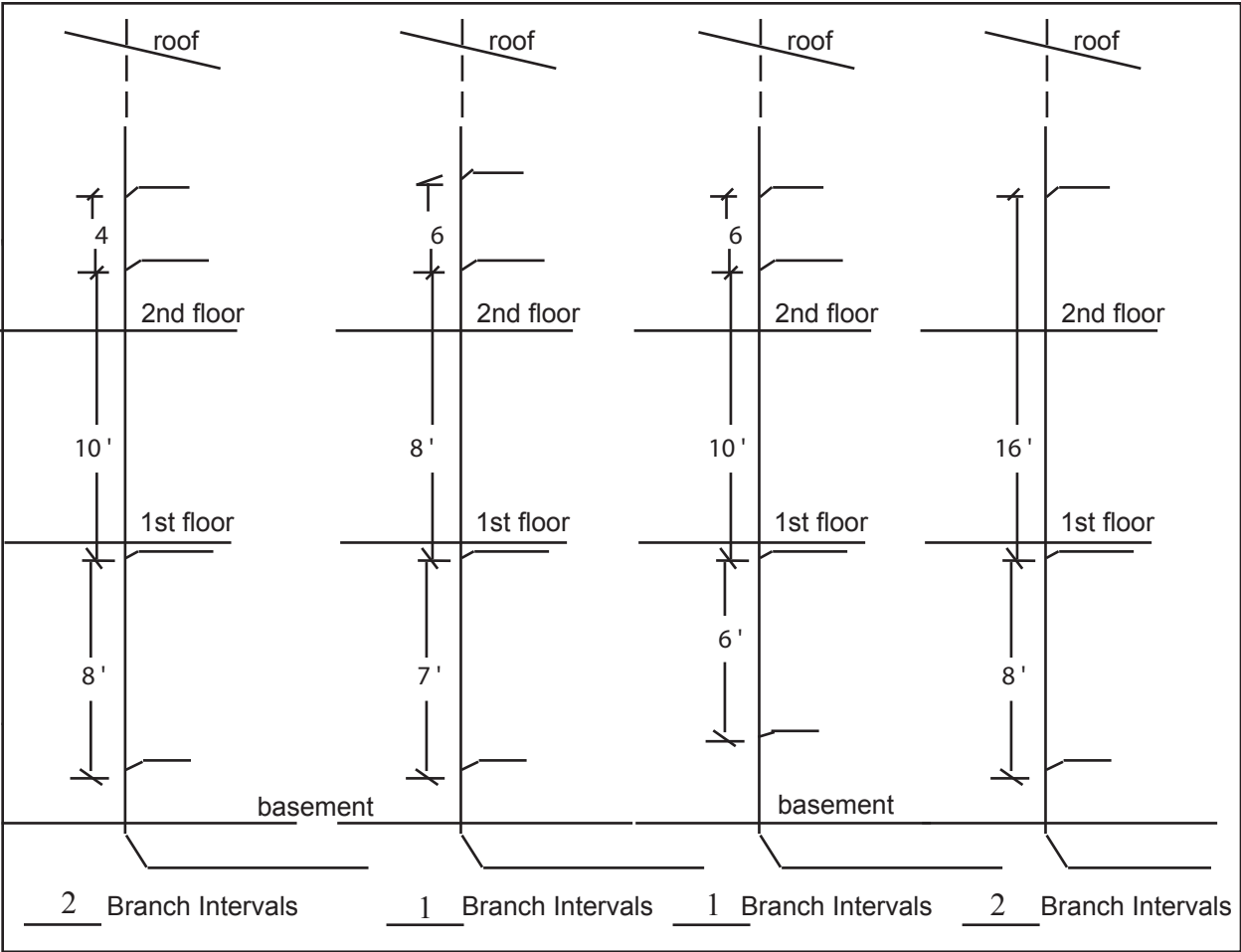
Answers to figure 7 worksheet. Measuring Branch Intervals.
