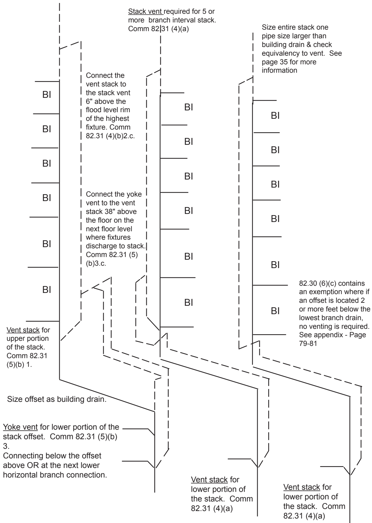
Figure 37. Three options: required vents for a horizontal offset below 5 branch intervals.
