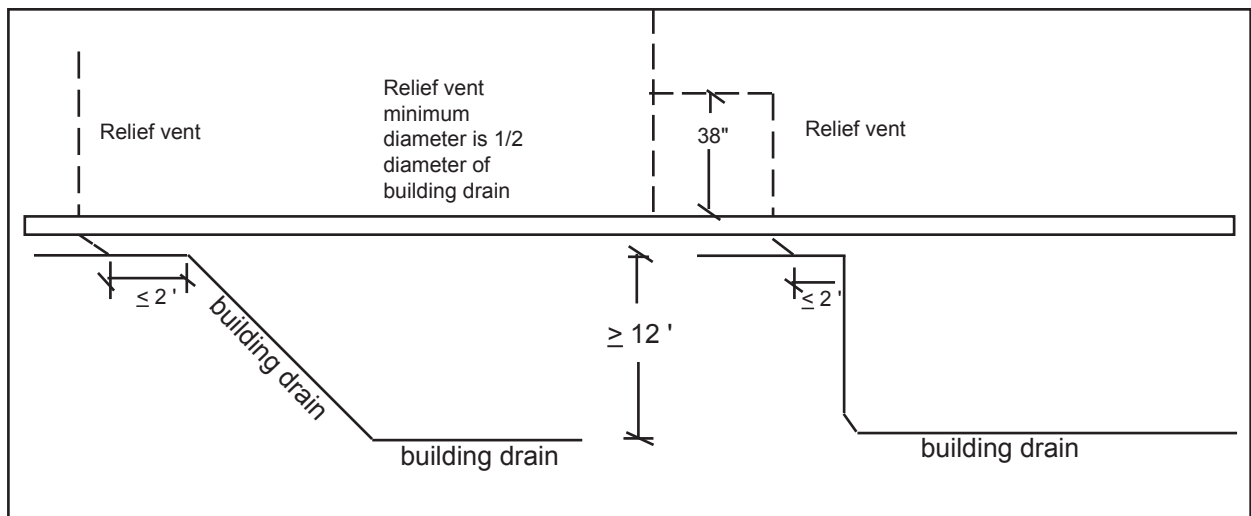
Figure 39. Relief vents for building drains
