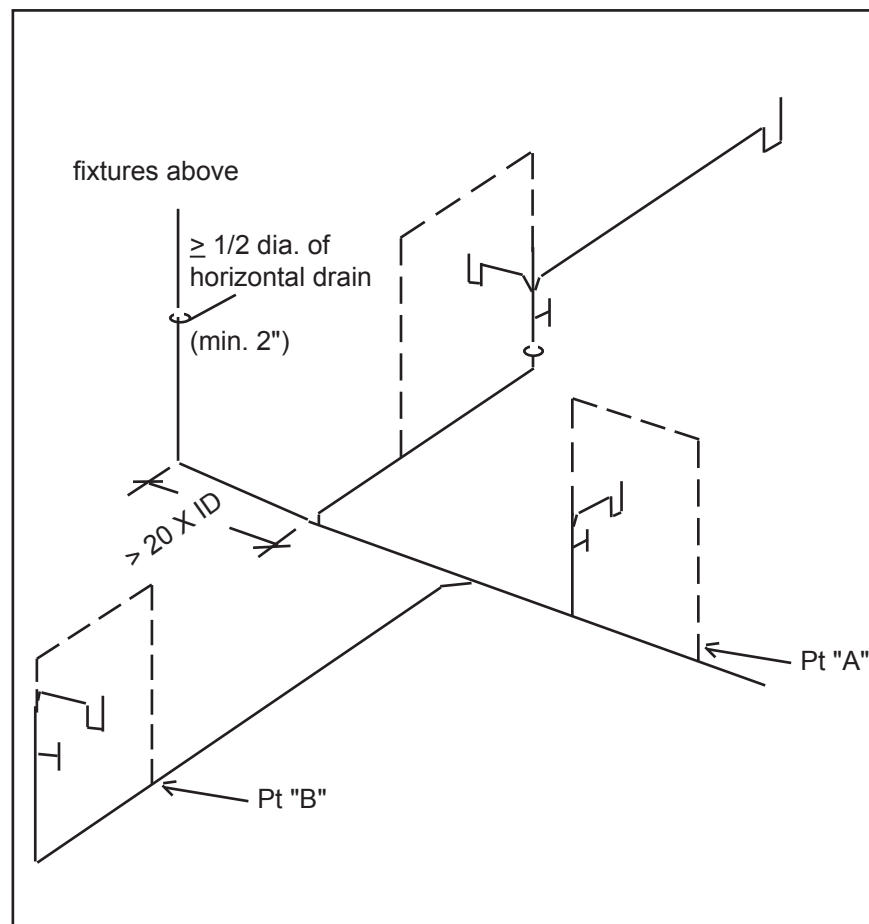
Figure 82. Laboratory sink combination drain and vent sizing
