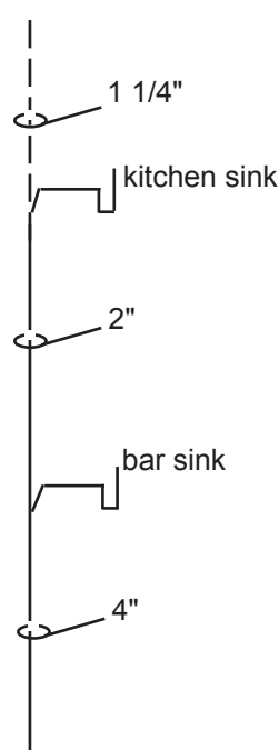
Figure 71. KS/bar sink stack
