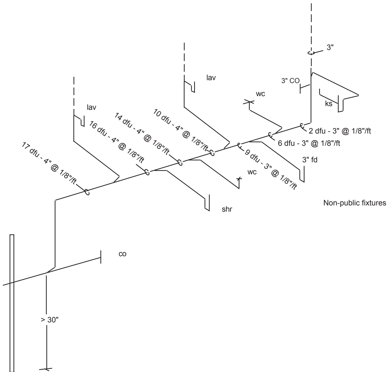
Figure 78. Combination drain and vent system design
