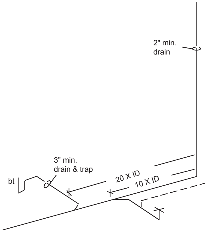
Figure 74. Combination drain and vent system and the building drain branch and horizontal branch drain.
