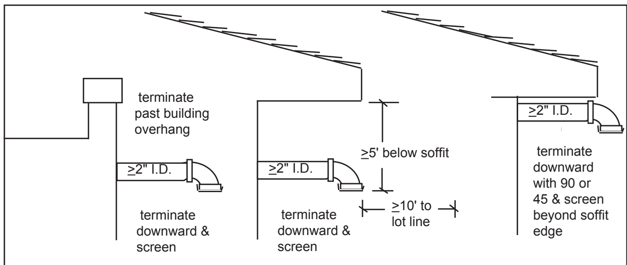
Figure 52. Vent terminal installation through exterior wall
