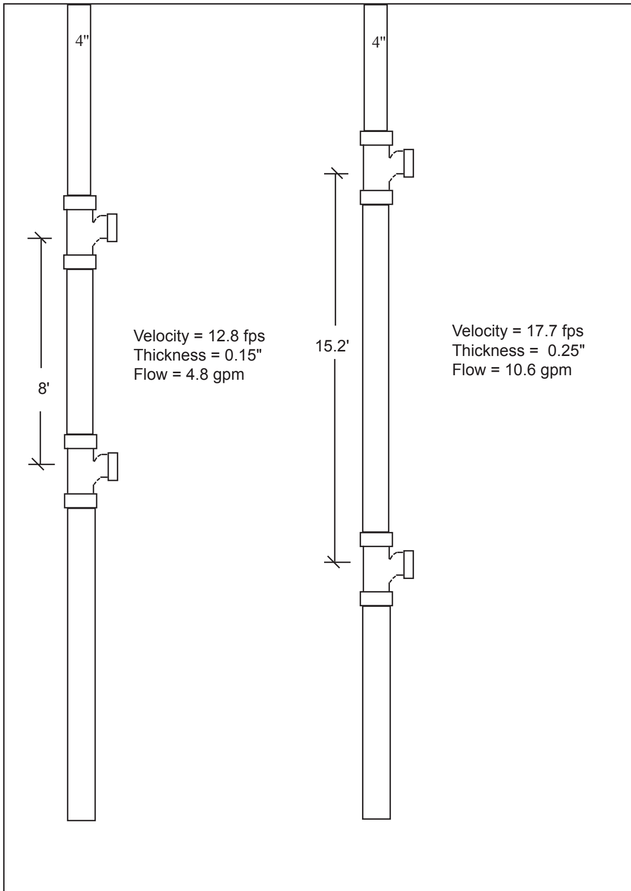
Figure 9 GPM load on stacks
