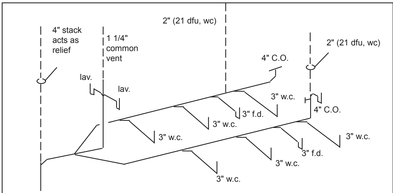
Figure 59. Circuit vent
