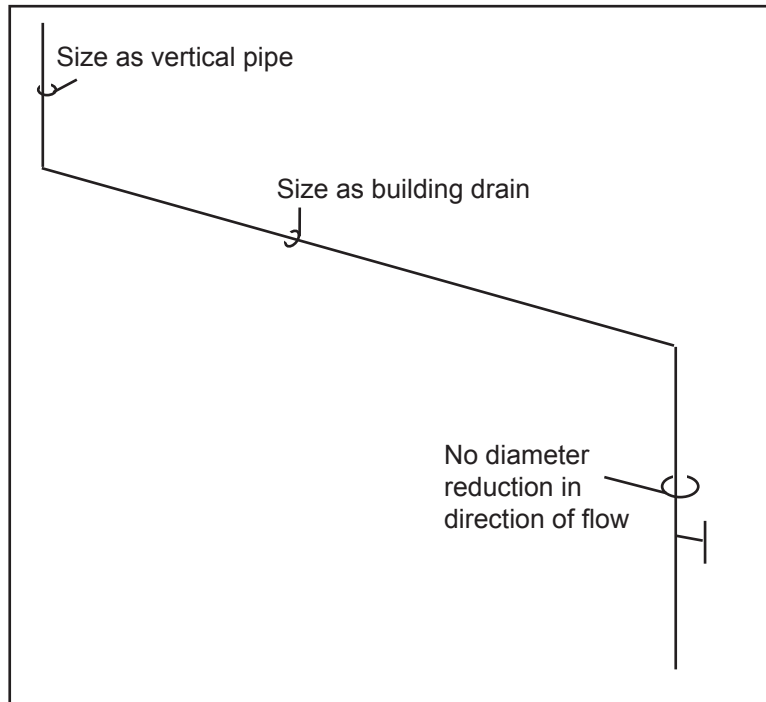
Figure 16. Minimum diameter for horizontal stack offsets.
