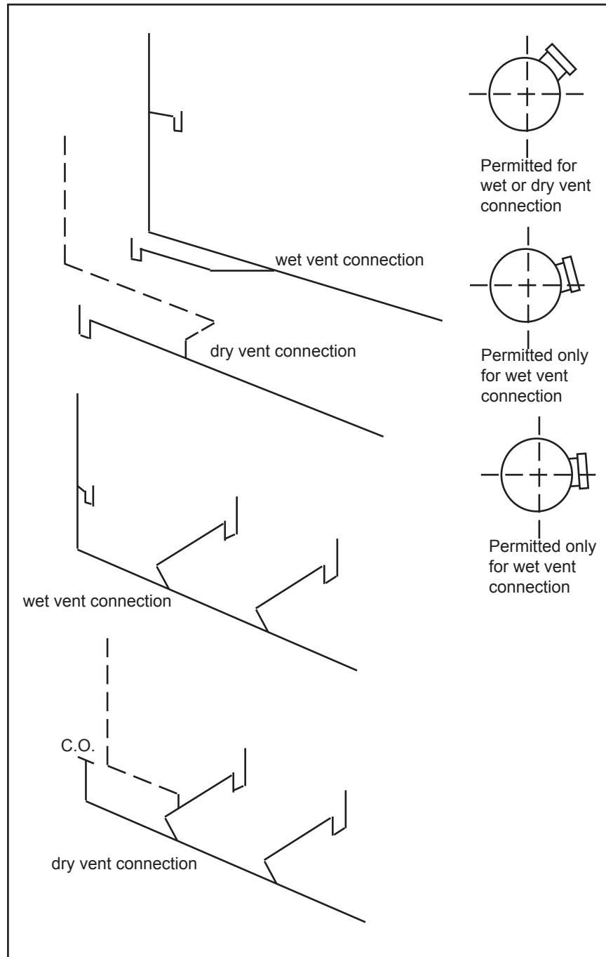
Figure 48. Wet and dry vent connections
