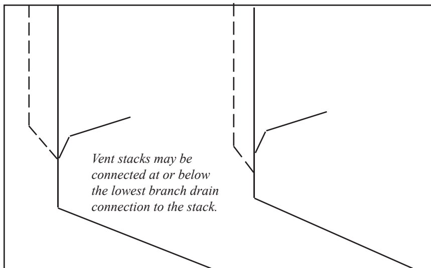
Figure 30. Connection of vent stack to drain stack
