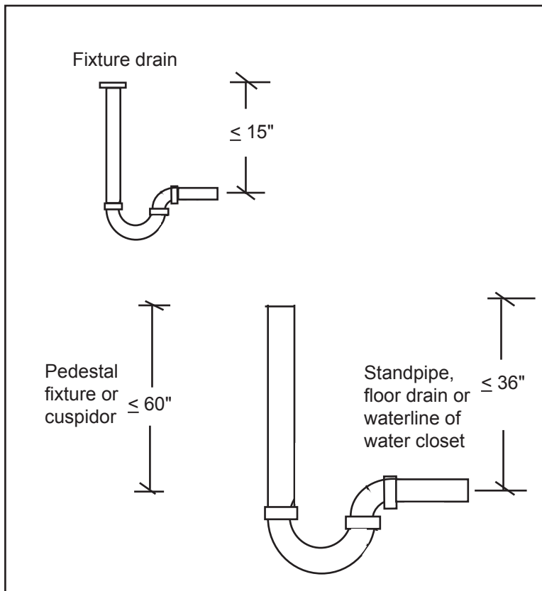
Figure 24. Vertical distance restrictions.
