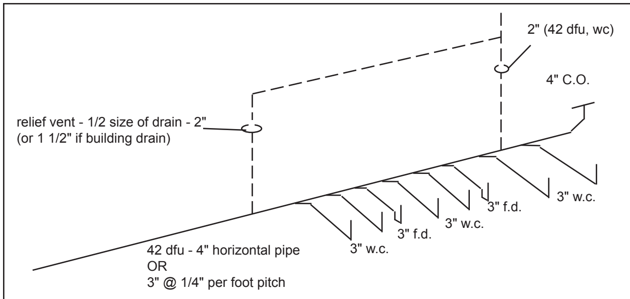
Figure 56. Circuit vent
