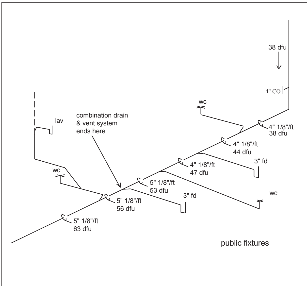
Figure 75. Combination drain and vent system
