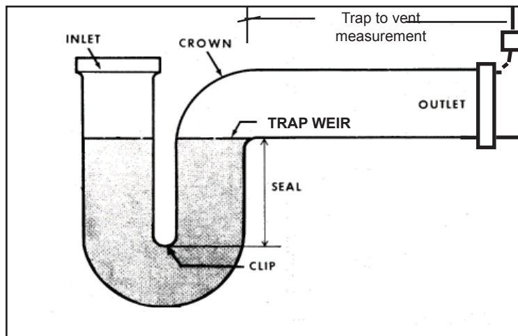
Figure 43. Vent to Trap Measurement
