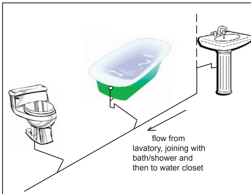
Figure 66. Flow through the horizontal wet vent
