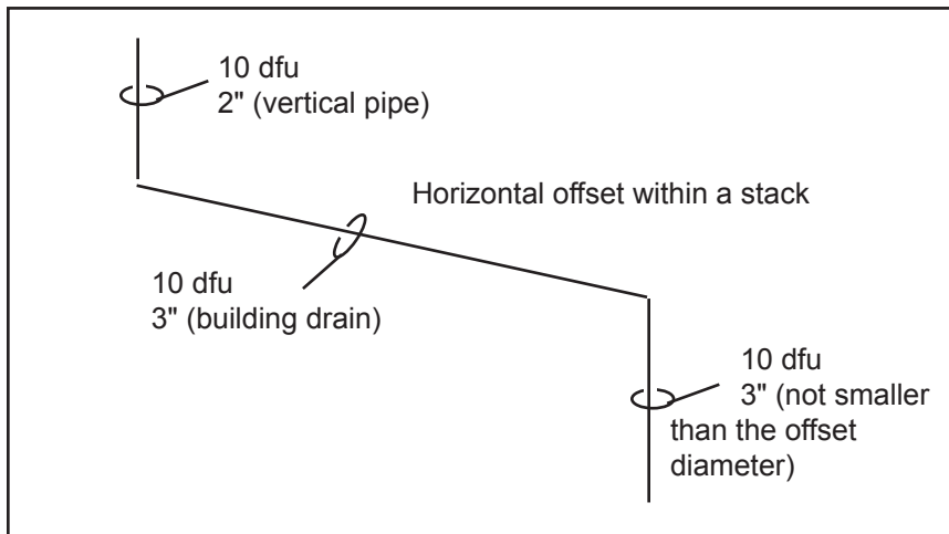
Figure 35. Horizontal offset - minimum diameters
