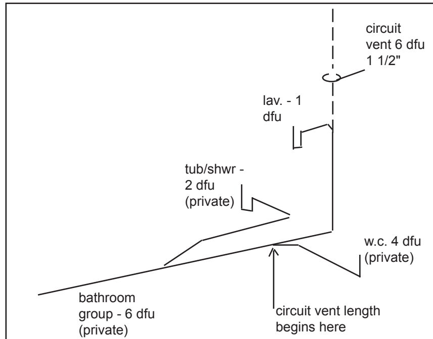
Figure 57. Circuit vented bathroom group
