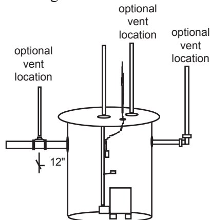
Figure 40. Vent placement options for sumps
