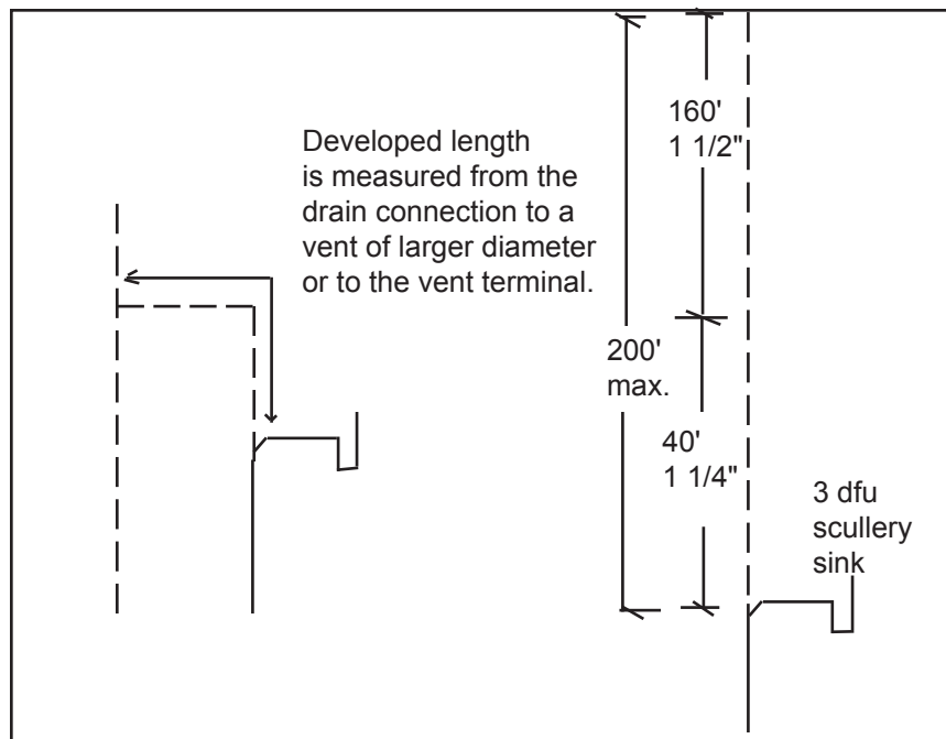
Figure 50. Determining vent diameter
