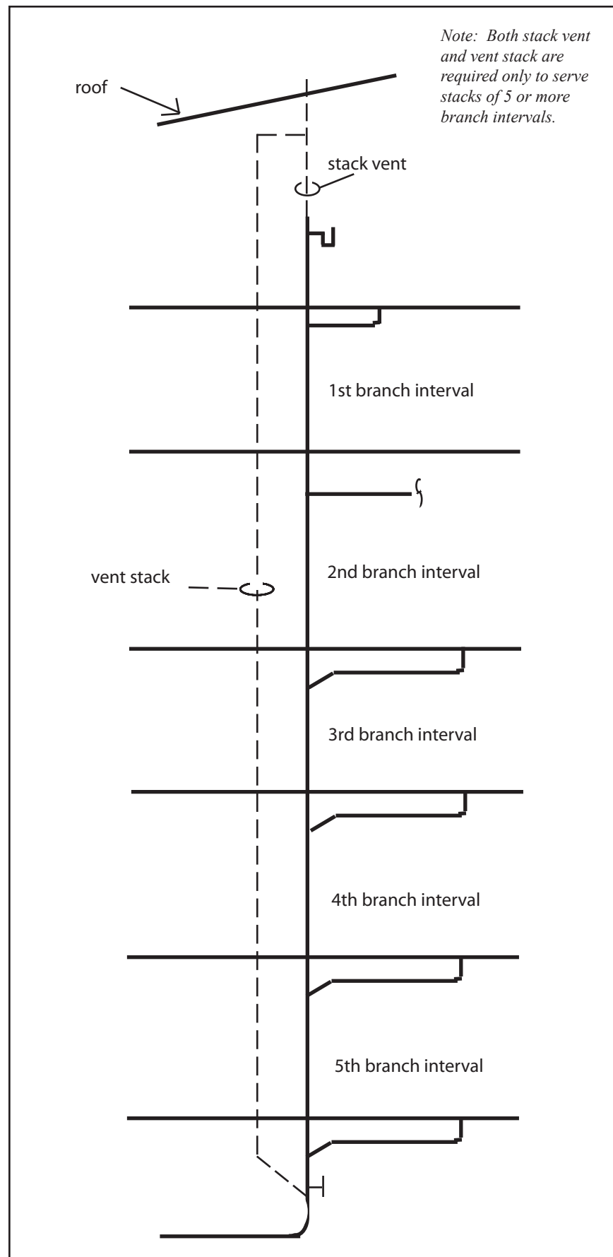
Figure 28. Vent Stack and Stack Vent
