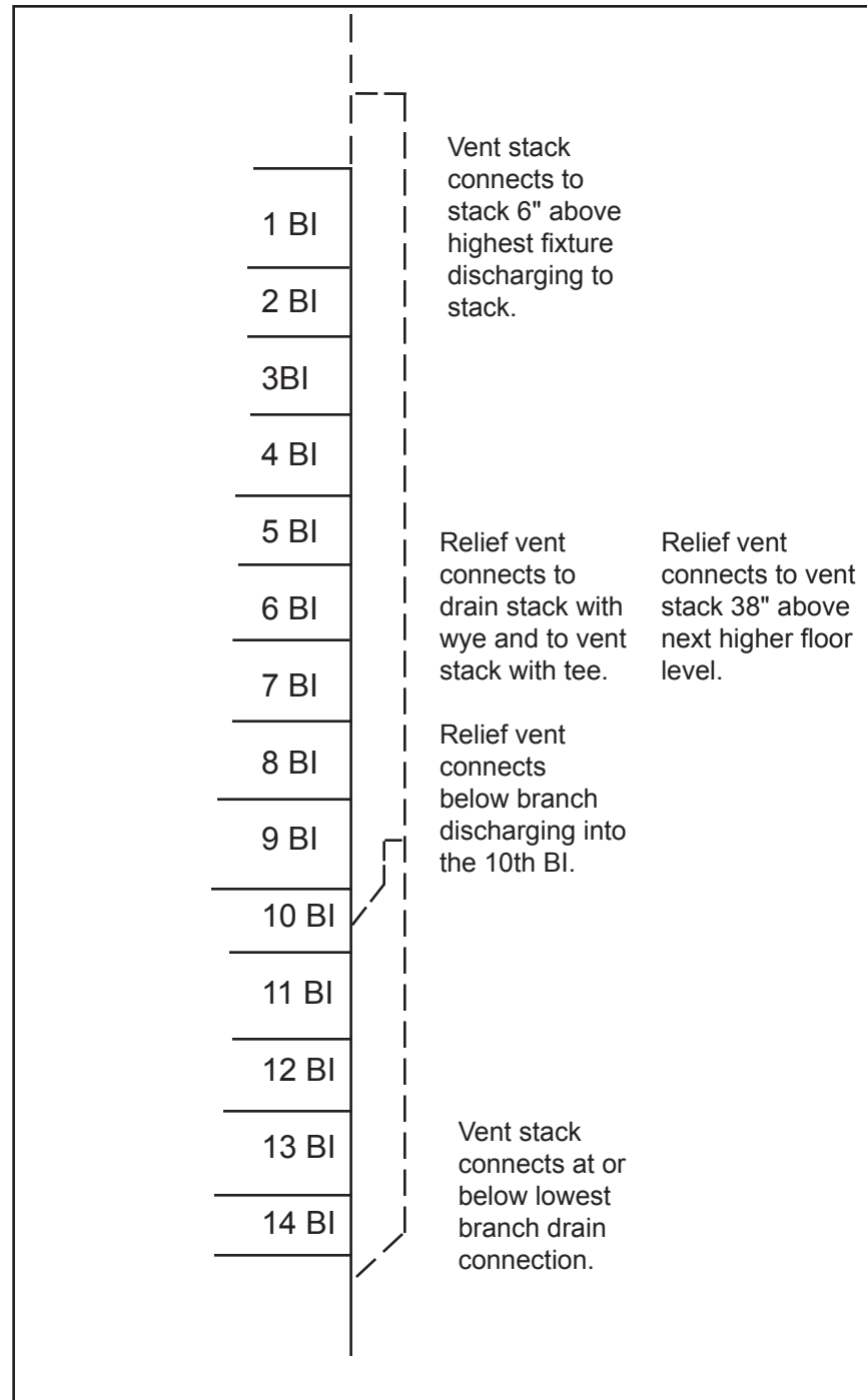
Figure 38. Relief vents for stacks of more than 10 branch intervals
