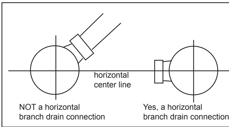
Figure 17. Connections above the horizontal centerline.
