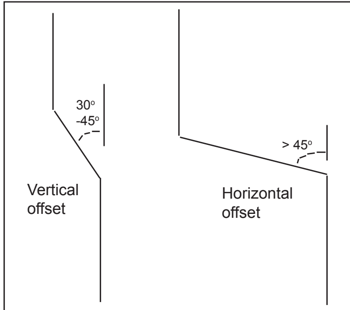
Figure 15. Types of stack offsets.
