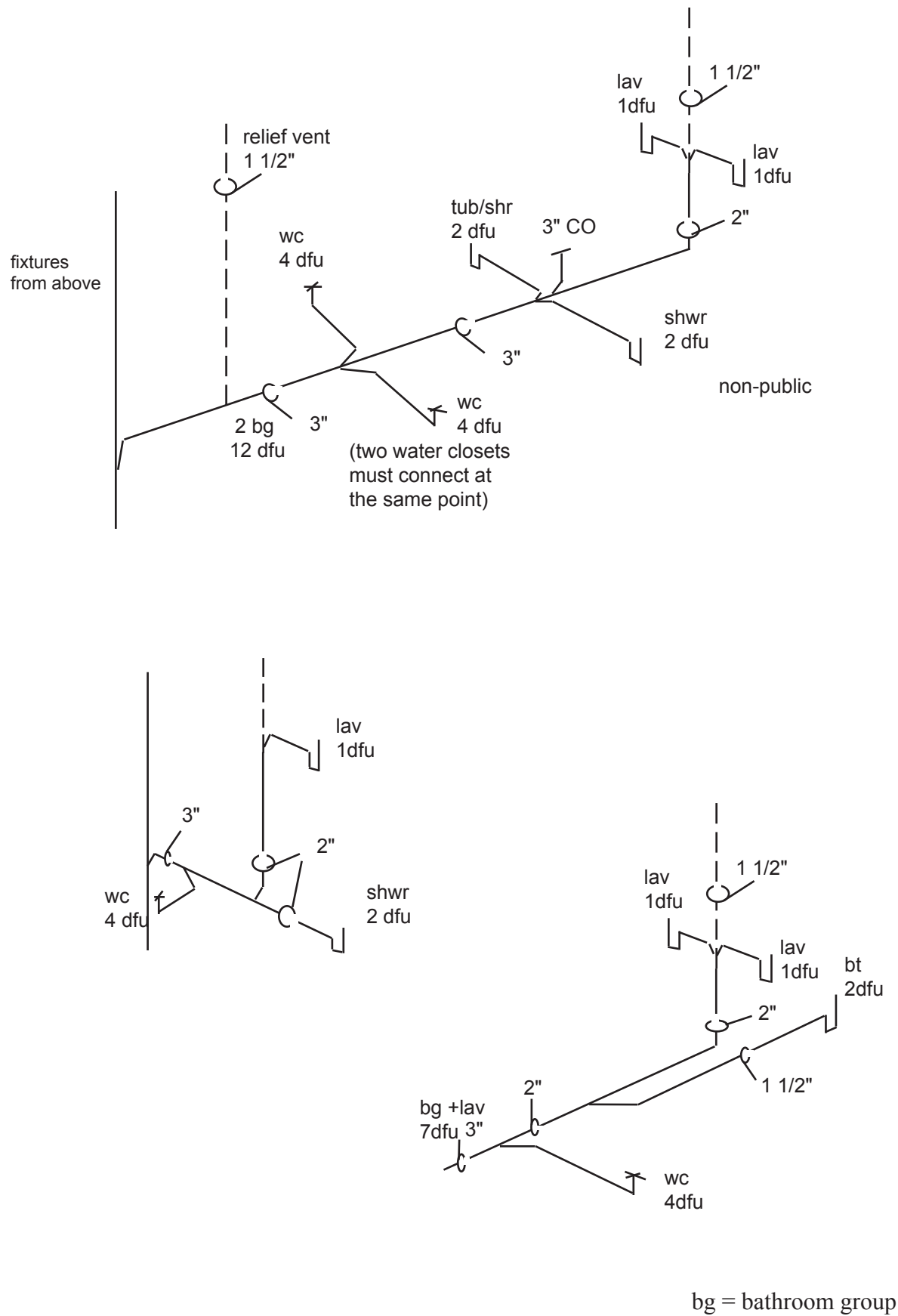
Figure 67. Examples of horizontal wet vent installations
