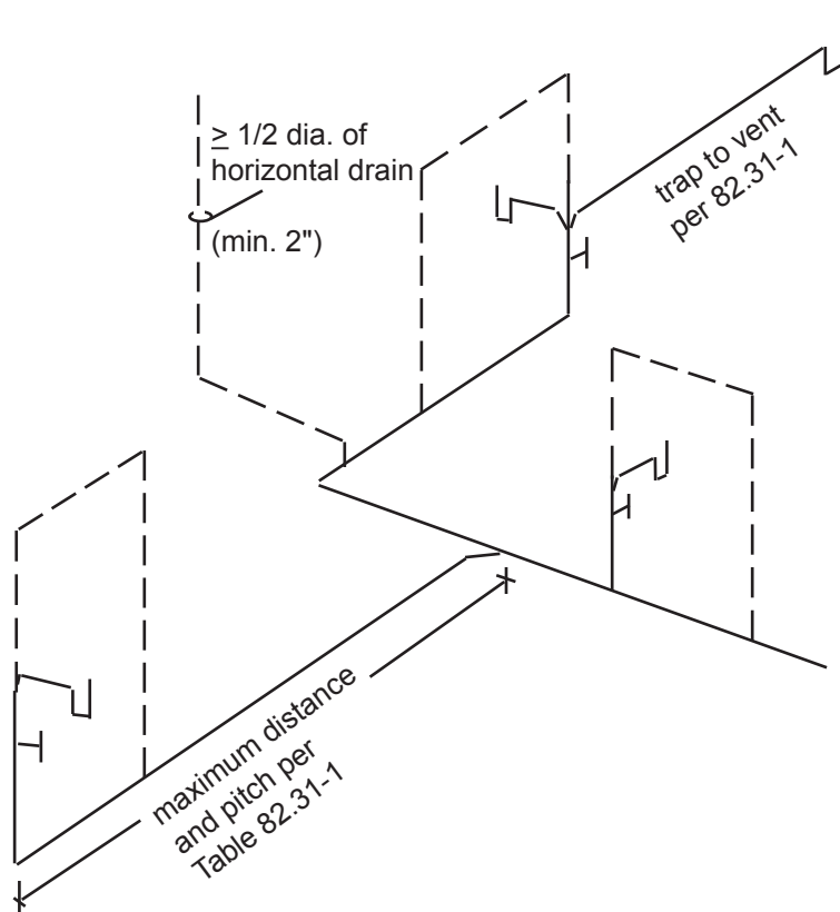
Figure 81. Combination drain and vent system
