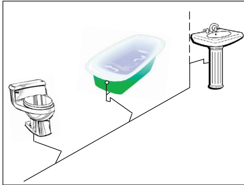
Figure 65. Horizontal wet vent
