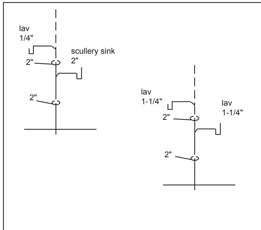
Figure 63. Vertical wet vent
