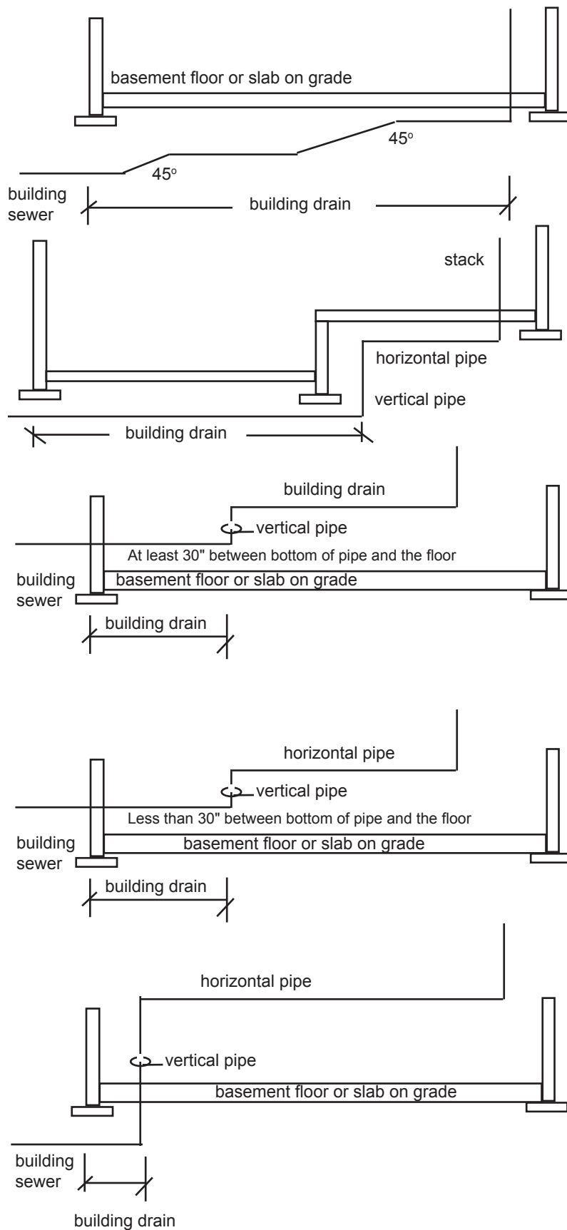
Figure 22. Designation of building drain piping.
