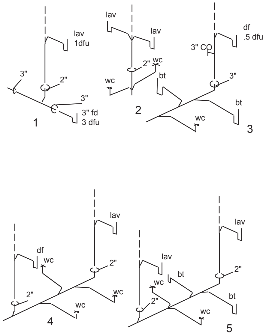
Figure 68. Wet vents
