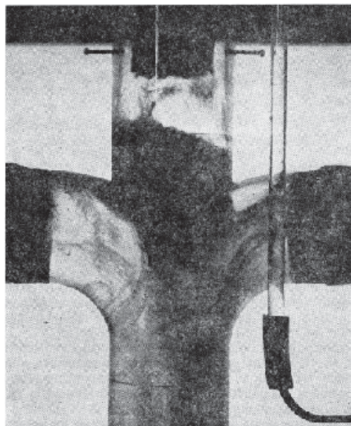
Figure 5. Flow into a 3-inch diameter stack from two horizontal branches at the same elevation, illustrating exceeding the capacity of the stack. NBS Monograph 31. July 3, 1961.
