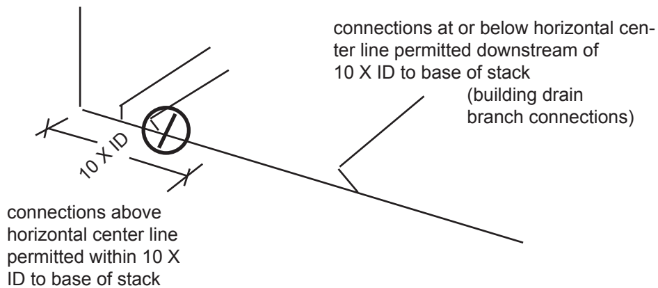
Figure 19. Connections at the base of a stack and connections at a stack offset
