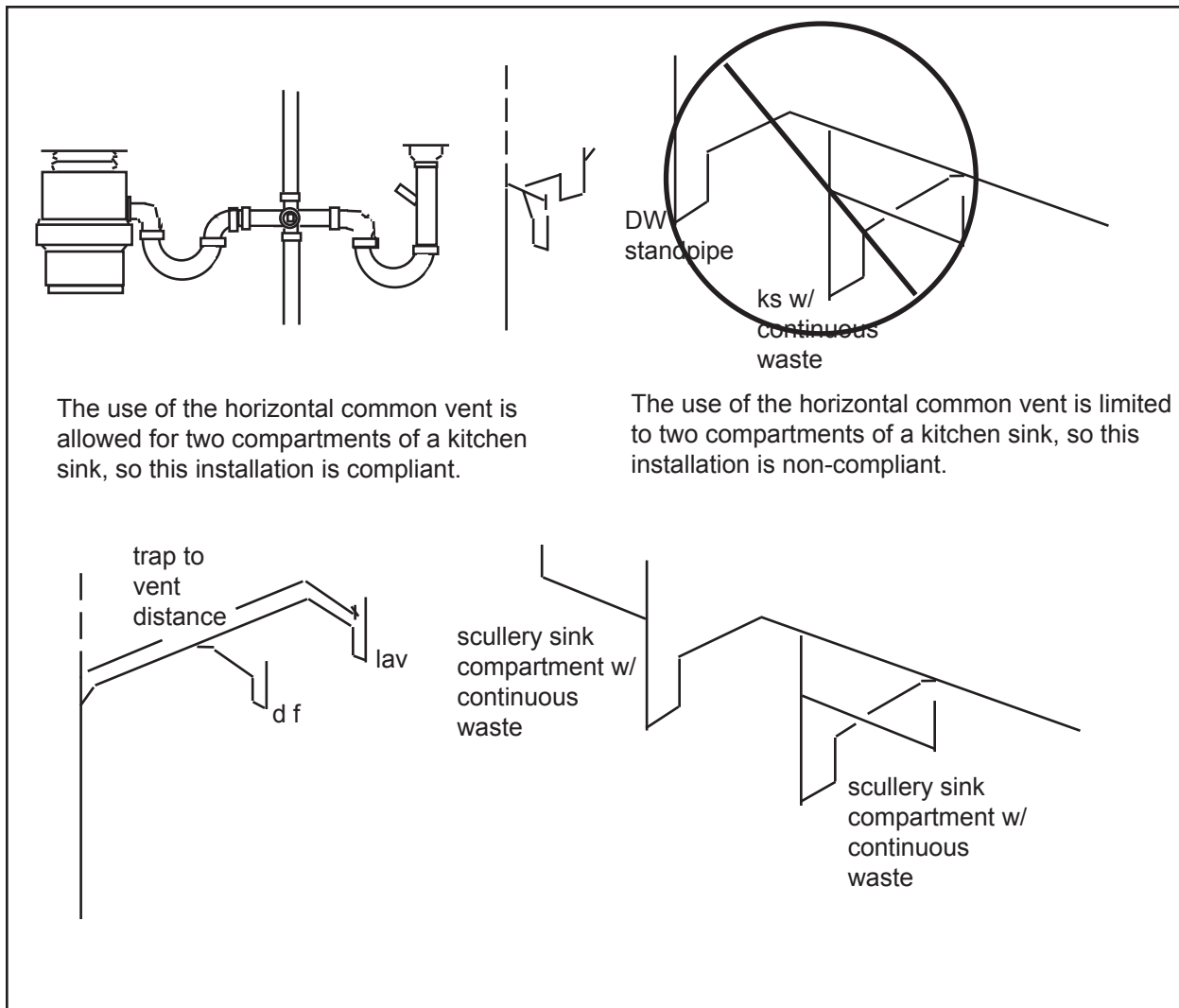
Figure 61. Horizontal common vent examples
