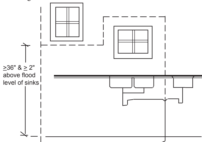
Figure 47. Vent drain, offset & connection requirements
