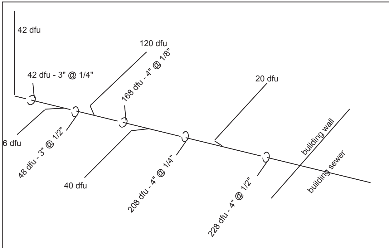
Figure 21. Building Drain Sizing
