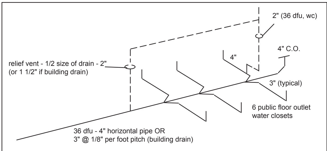
Figure 55. Circuit vent
