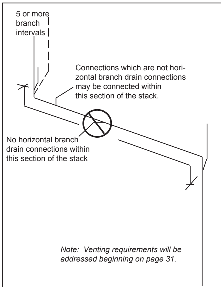
Figure 18. Connections to offsets below 5 or more branch intervals.
