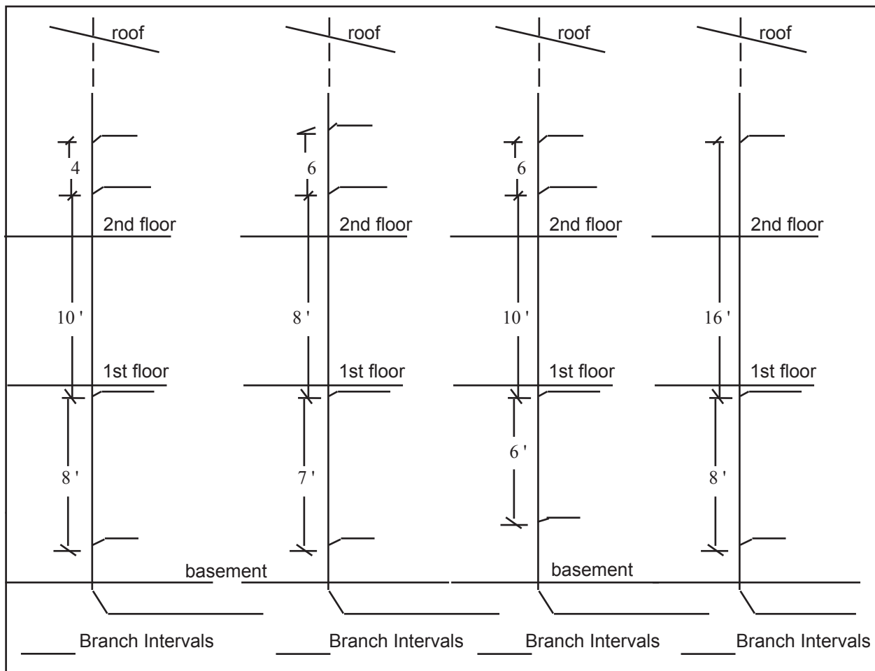
Figure 7. Measuring Branch Intervals
