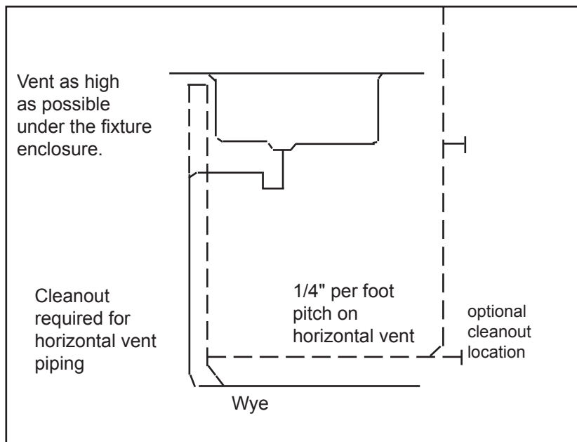
Figure 62. Return Vent
