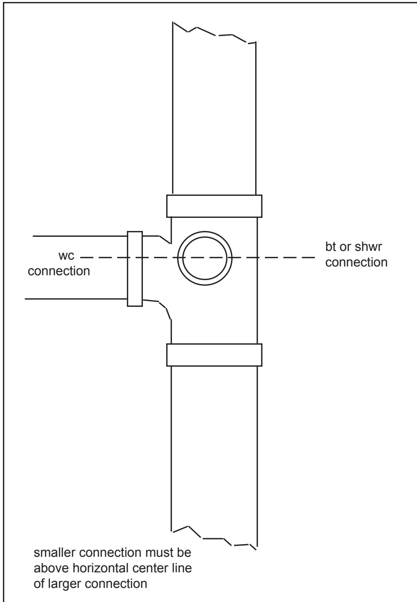
Figure 60. Vertical common vent with side inlet tee
