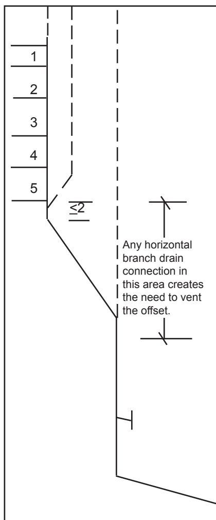
Figure 33. Venting a 45° offset
