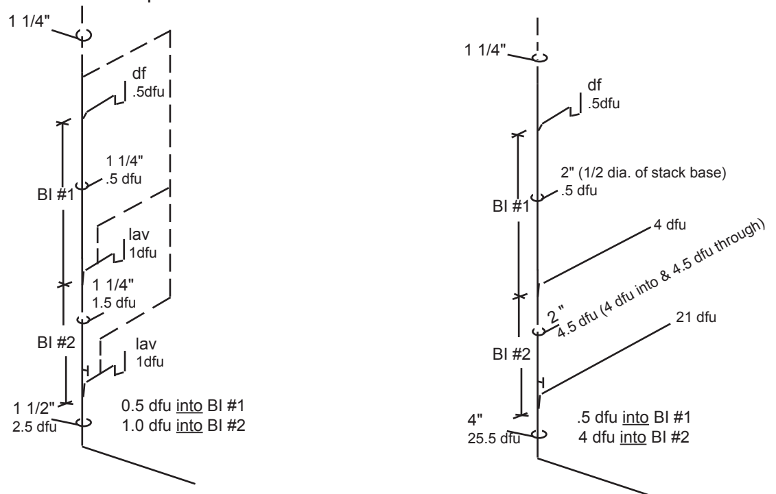
Figure 12. Sizing Stacks
