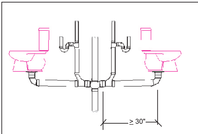
Figure 27. Branch drain connections with water closets
