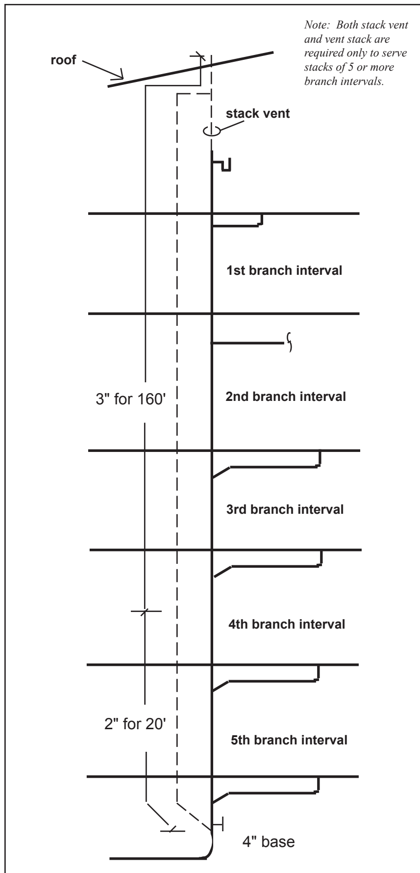
Figure 31. Vent Stack Sizing
