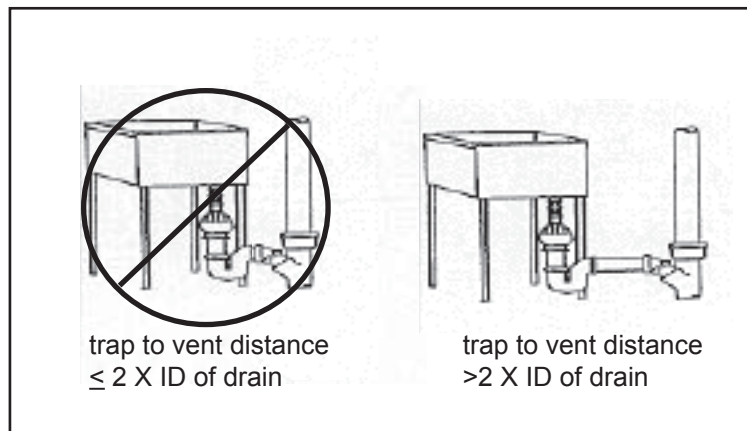
Figure 45. Minimum trap to vent distance
