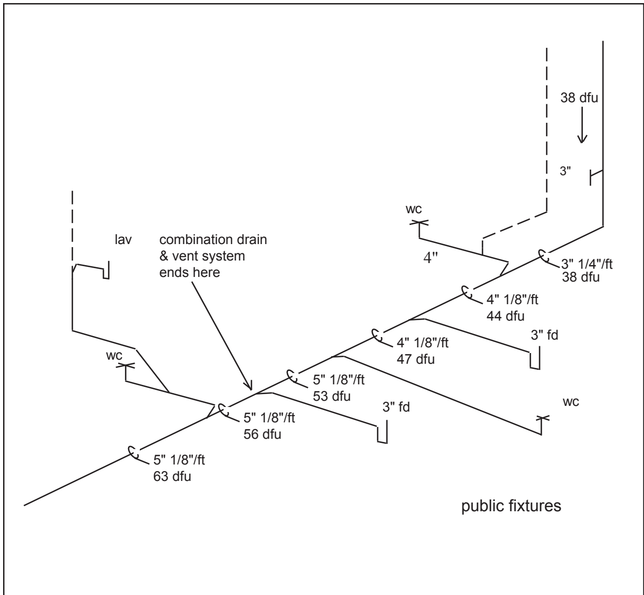
Figure 76. Combination drain and vent system
