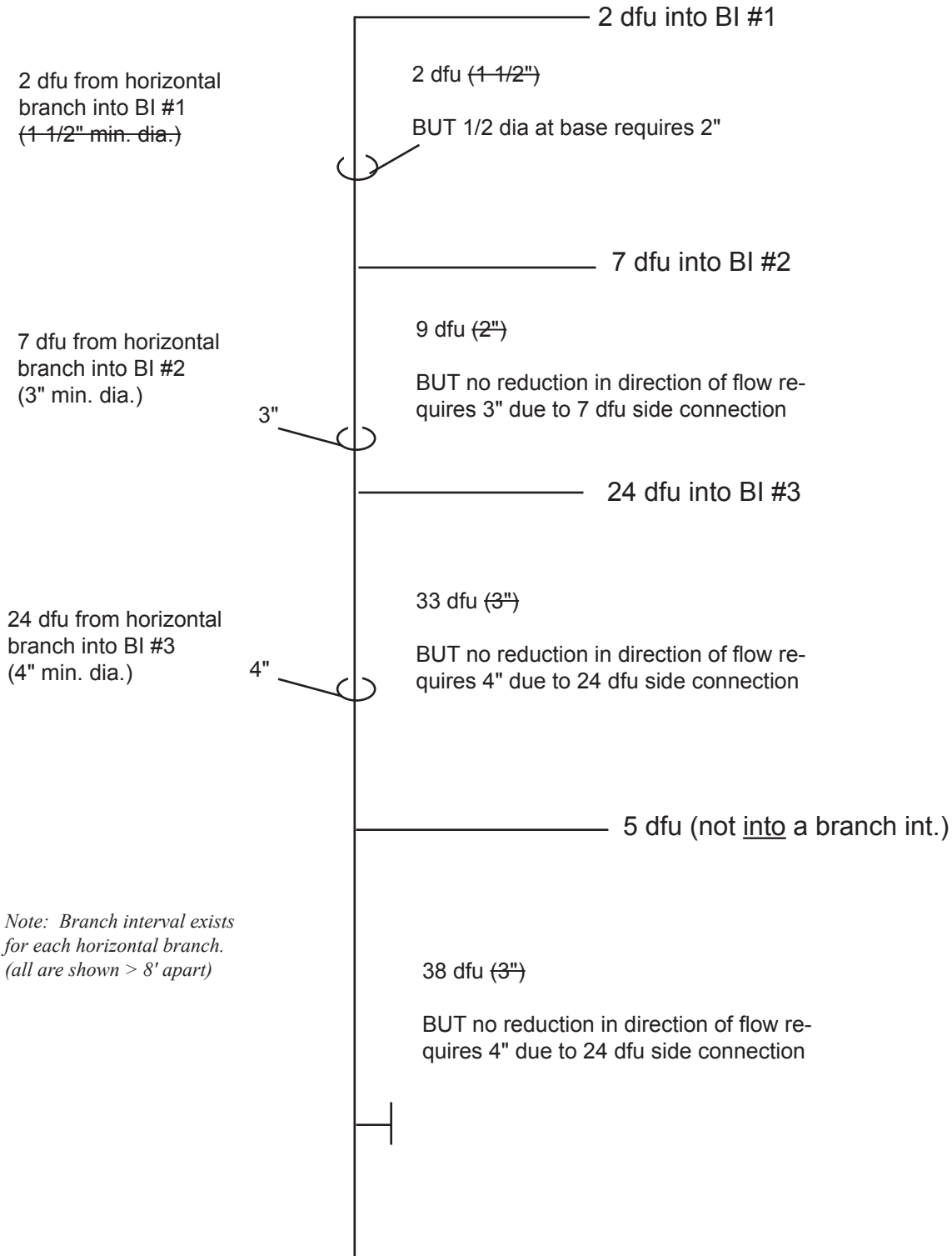
Figure 13. How horizontal branch drains affect minimum stack diameter
