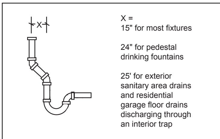
Figure 25. Horizontal distance restrictions.
