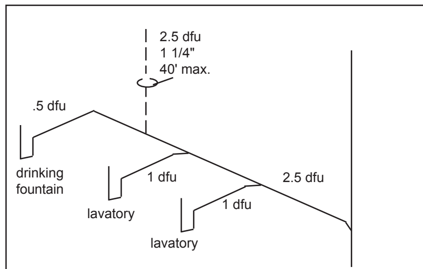
Figure 54. Circuit vent design
