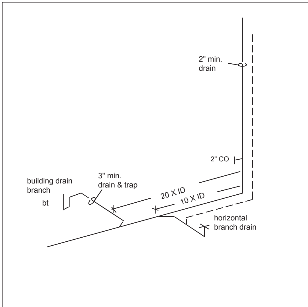
Figure 74. Combination drain and vent system utilizing the building drain
