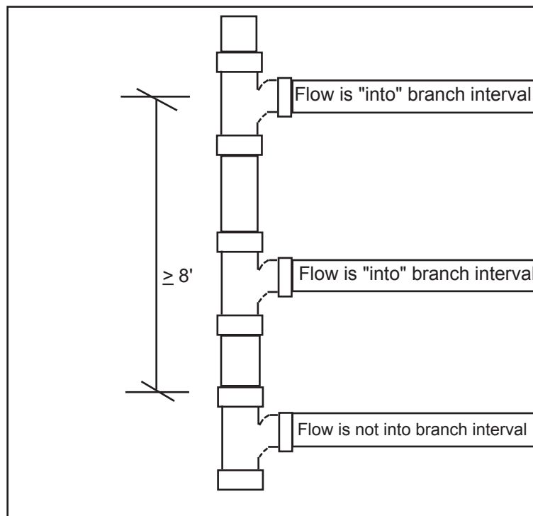
Figure 11. Into and Through the Branch Interval
