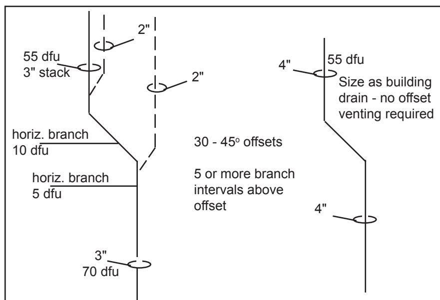
Figure 34. Two methods for venting a stack offset below 5 branch intervals
