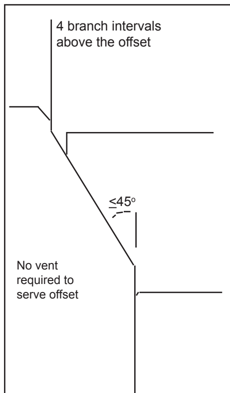
Figure 32. Vertical Offset < 5 BI
