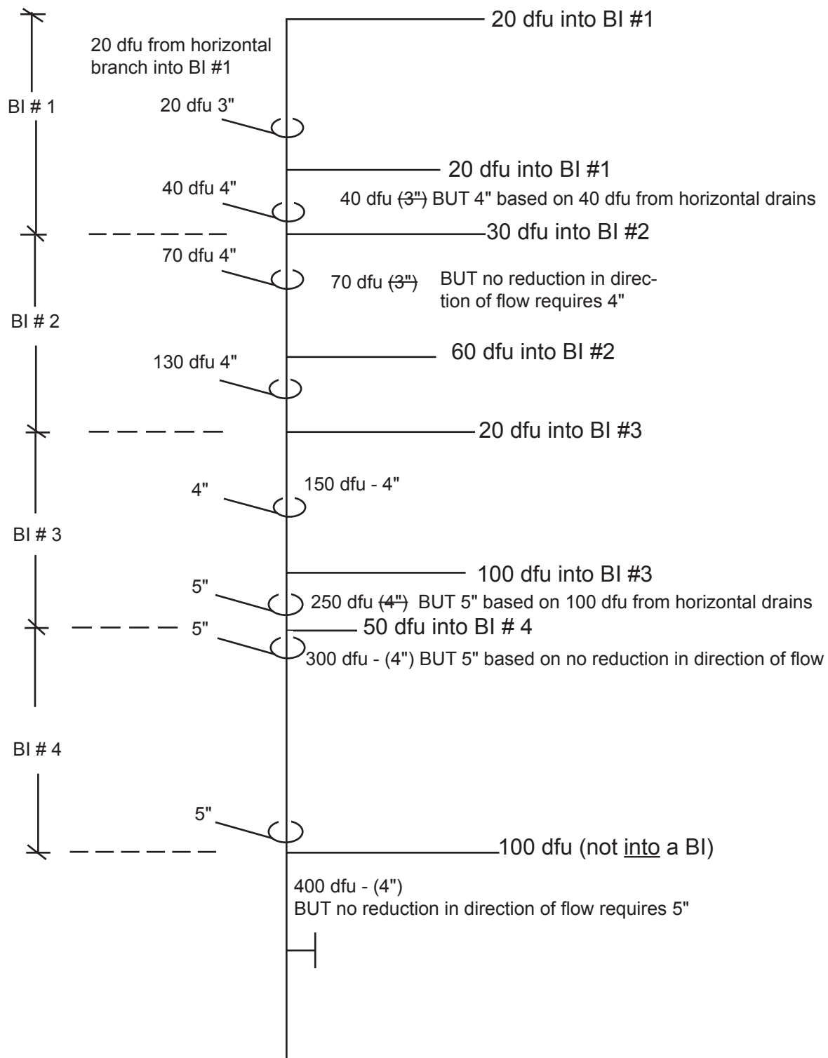
Figure 14. How horizontal branch drains affect minimum stack diameter
