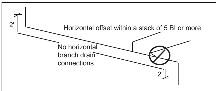
Figure 36. Connections to horizontal offset below 5 or more branch intervals.
