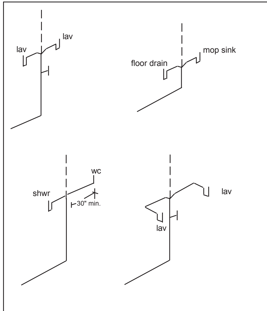
Figure 59. Common vent
