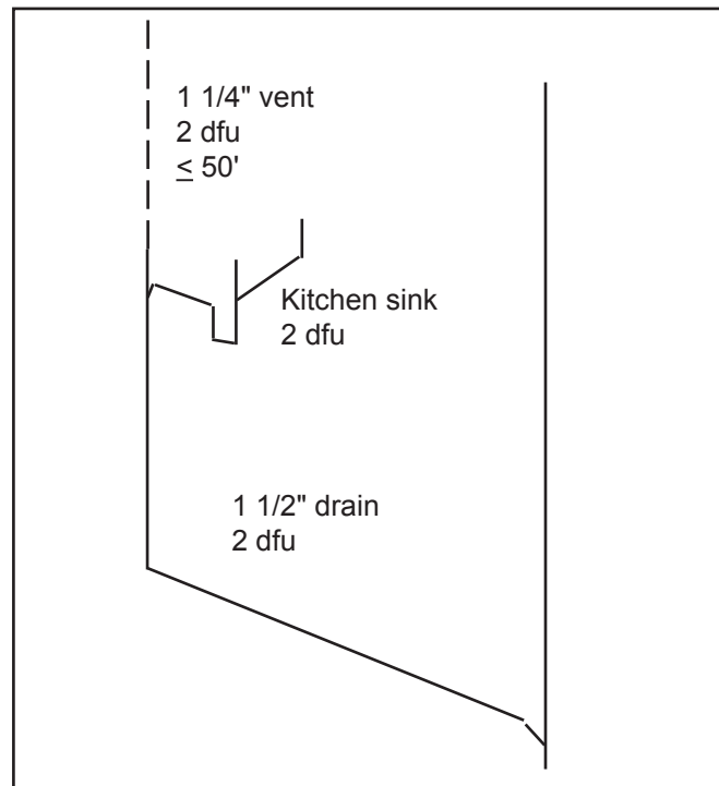
Figure 53. Individual vent design
