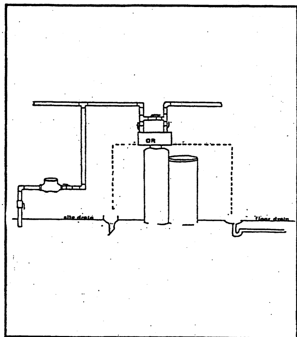
Figure 3-10: Discharge of softener backwash to sanitary or storm
