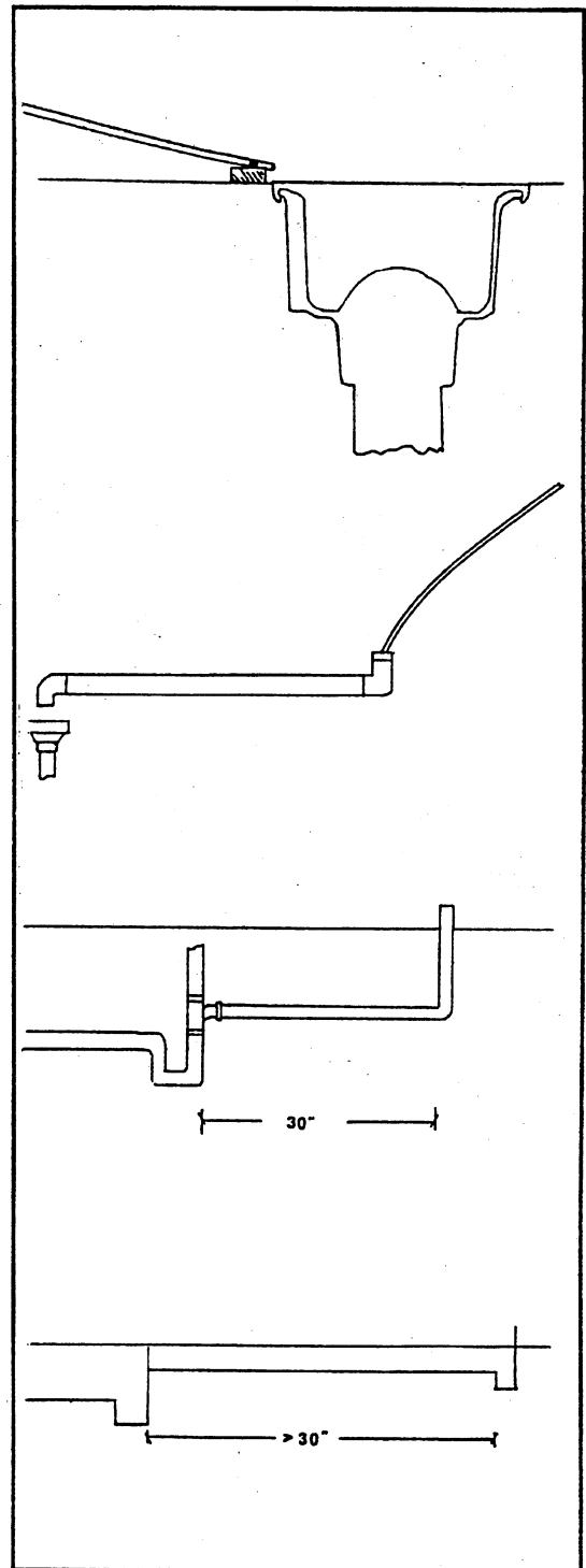
Figure 2-9: Approved air gap installations
