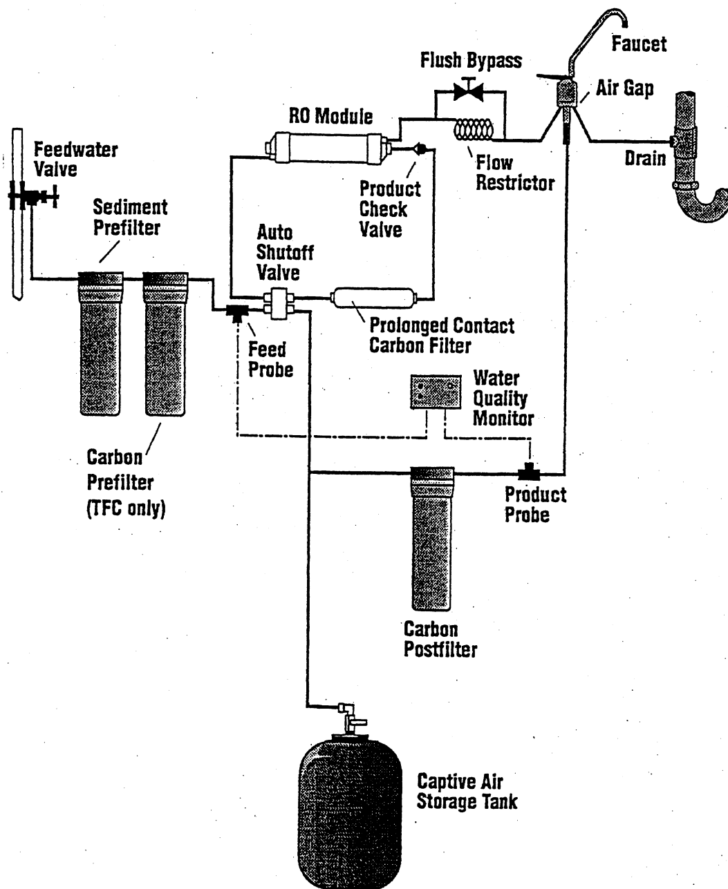
Figure 4-5: Typical under-cabinet installation Courtesy of Water Factory Systems
