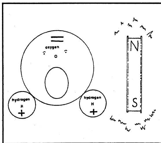
Figure 1-1: Water, the dipolar molecule
