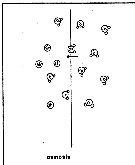
Figure 1-8: Osmosis
