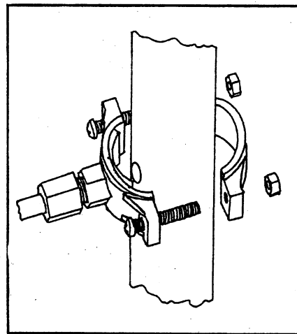
Figure 2-12: Approved drain saddle fitting
