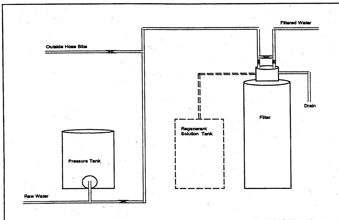
Figure 5-3: Manganese treated mineral filter on a private well.
