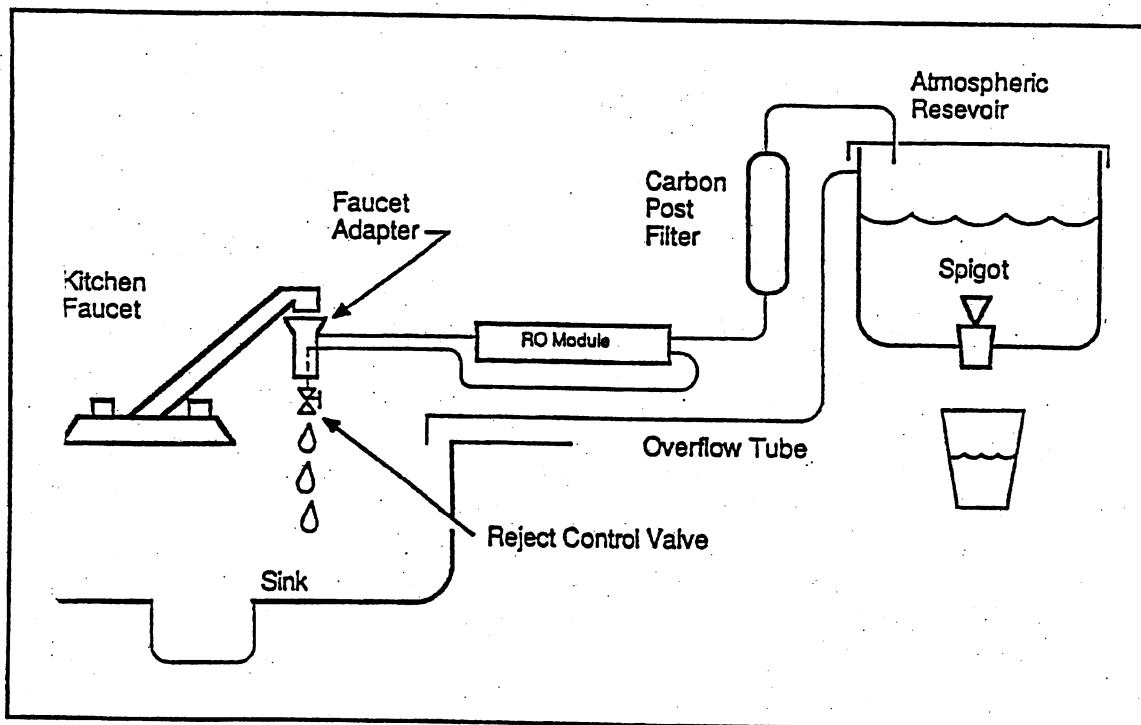
Figure 4-6: Typical countertop installation. Courtesy of Water Factory Systems
