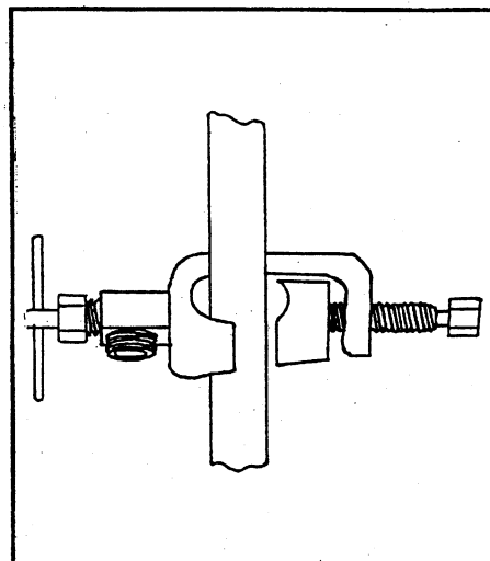
Figure 2-5: Self-tapping saddle for water supply
