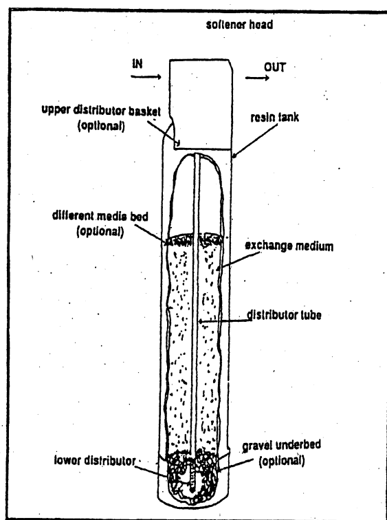
Figure 3-9: Exchange tank design
