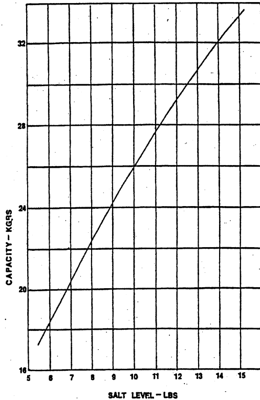
Figure 3-7: Efficiency curve as the salt concentration is increased for a particular size of softener
