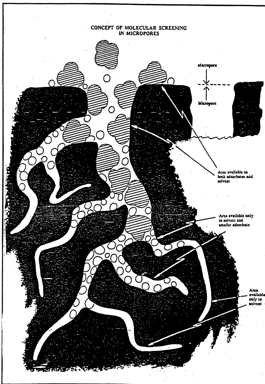
Figure 6-1: The porous surface of activated carbon.
