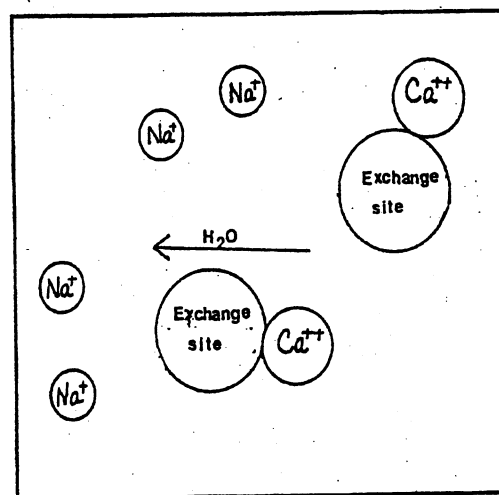
Figure 3-4: The more calcium (or magnesium) in untreated water, the more sodium in treated water
