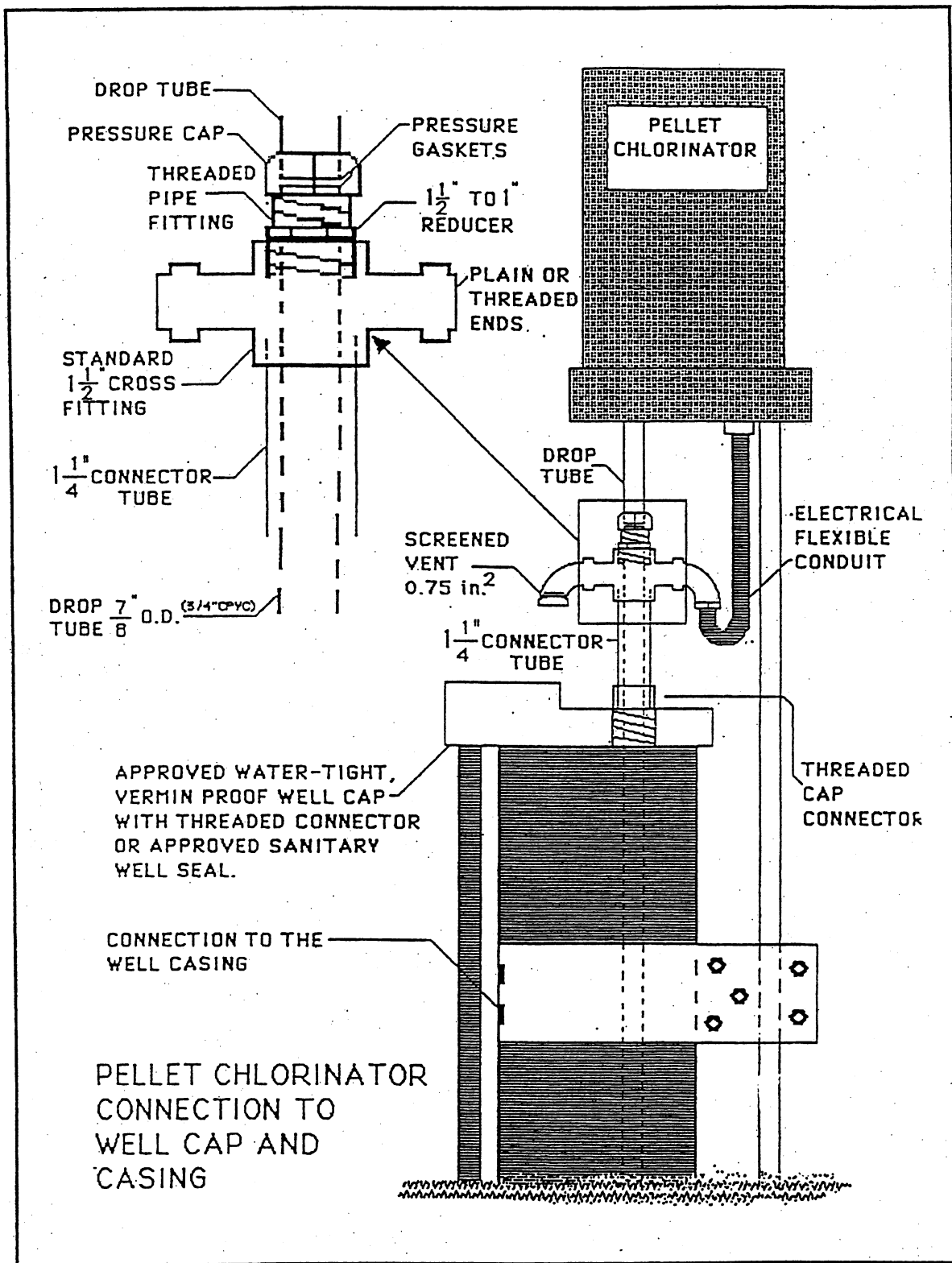
Figure 5-2: Pellet chlorinator installation guidelines.
