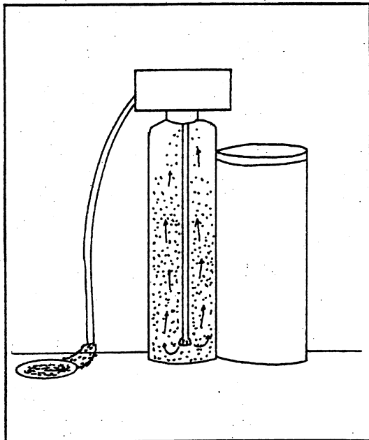
Figure 3-5: High flow rates can push medium out of mineral tanks
