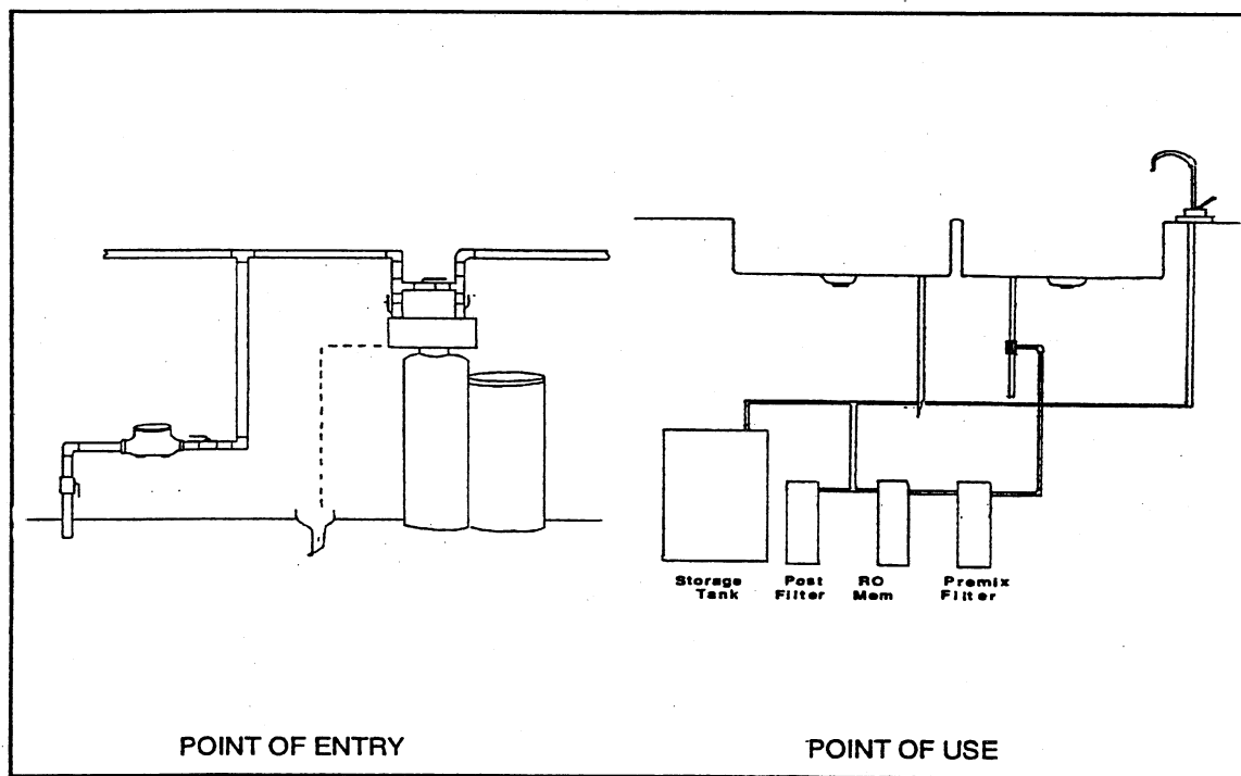
Figure 2-2: Point-of-Entry and Point-of-Use
