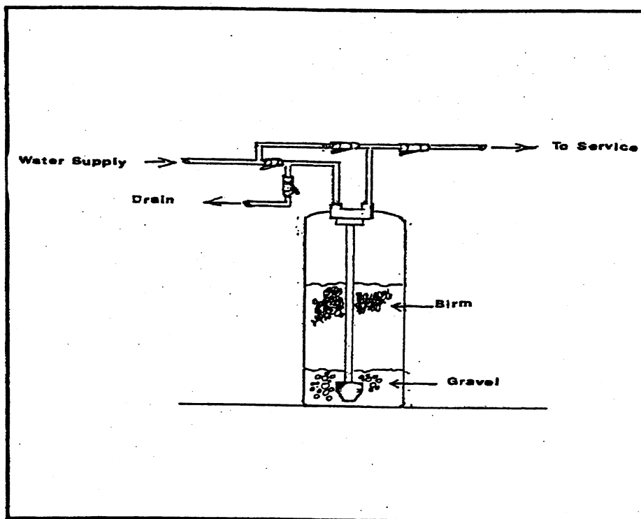
Figure 5-4: Catalytic Filter
