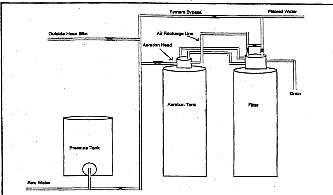
Figure 5-1: Aeration used for oxidation of iron prior to filtration.
