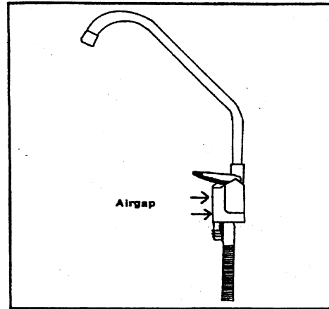
Figure 2-11: Internal air gap
