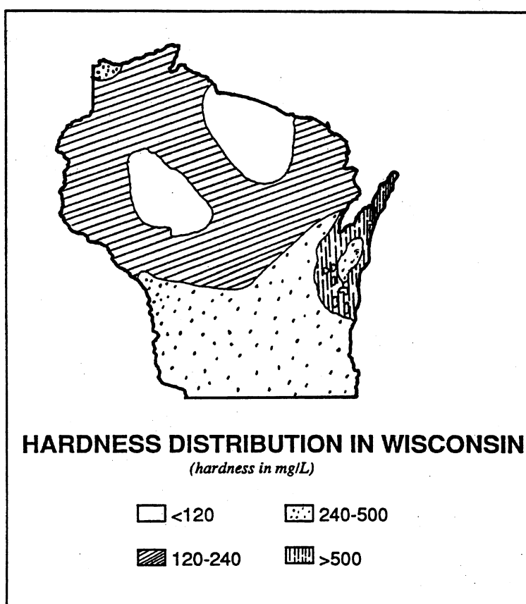
Figure 1-10: Hardness of Wisconsin's Groundwater
