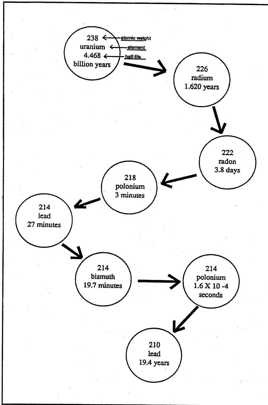
Figure 1-11: The decay chain of radon (LaFavore 1987)
