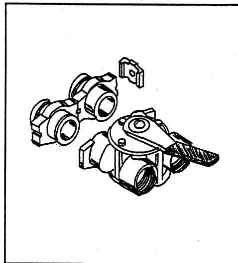
Figure 2-7: Approved internal bypass
