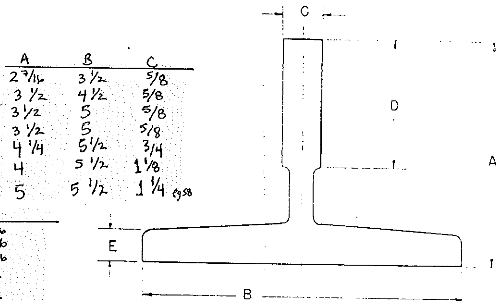
FIGURE 4.55 ELEVATOR GUIDE RAILS
